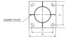
BASE PLATE FOR POLE HEIGHTS ABOVE 12 METERS
