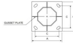
BASE PLATE FOR POLE HEIGHTS ABOVE 12 METERS
