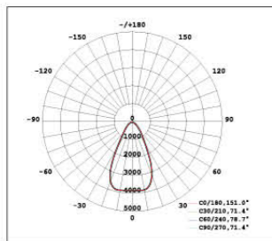
60° lighting distribution
